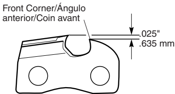
Figure 22 - Round Off Front Corner Of Depth Gauge
